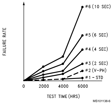
FIGURE 3. Immersion in 360°C Solder
