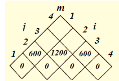
MATRIX-CHAIN-ORDER(p)
