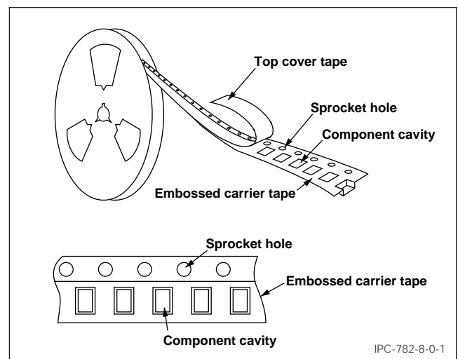
Figure 1 Packaging
