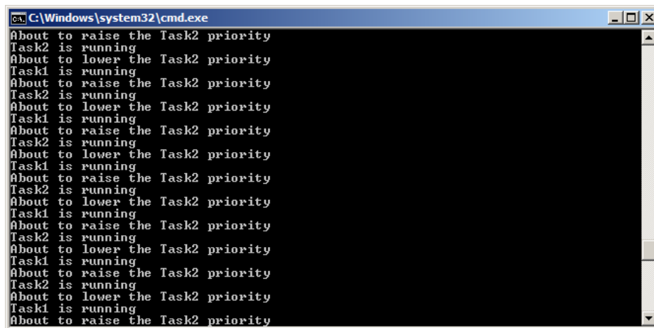
Figure 23. The output produced when Example 8 is executed
